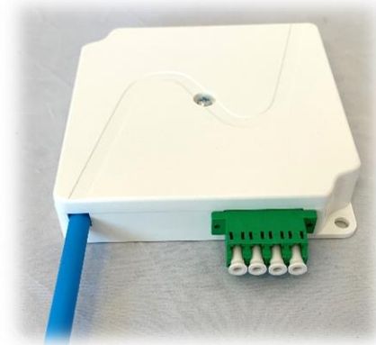
7/3,5 mm microduct and 4F micro cable installed to Nestor OptoBox 4 LC/APC 4xSMT pigtail kit
