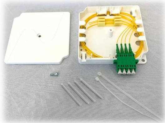
Nestor OptoBox 4 LC/APC 4xSMT pigtail kit
